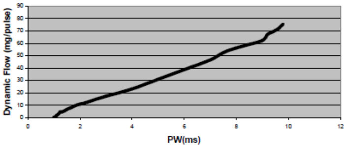
Characteristic Injector Flow Curve
