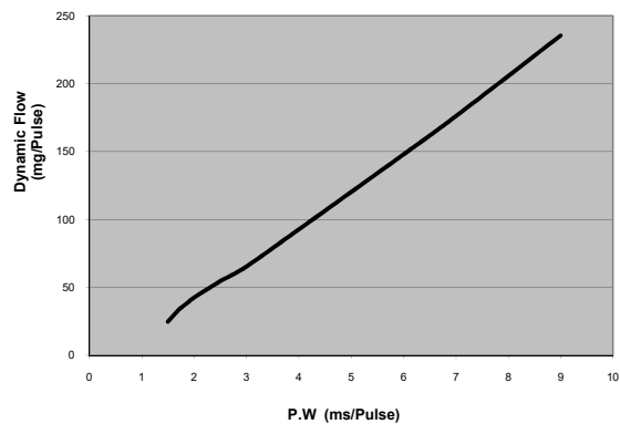
Characteristic Injector Flow Curve
